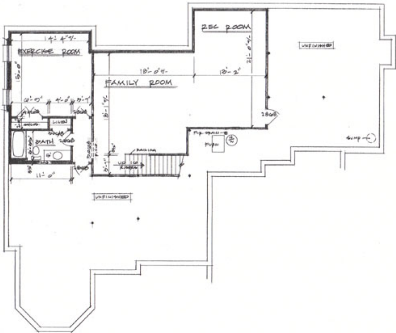
BASEMENT PLAN 1/4" = 1'-0" 1,100 #7 - FINISHED
