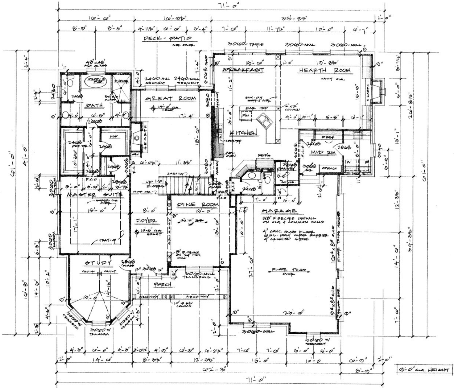
FIRST FLOOR PLAN 1/4" = 1'-0" 2,050 #7-
